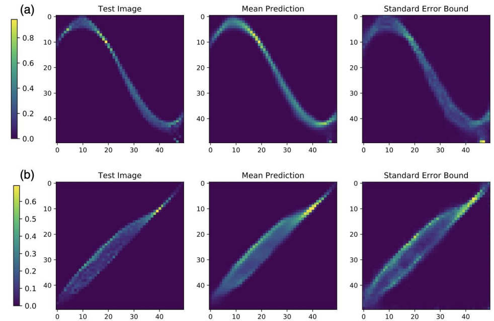
LCLS-II longitudinal phase space simulations predictions.
