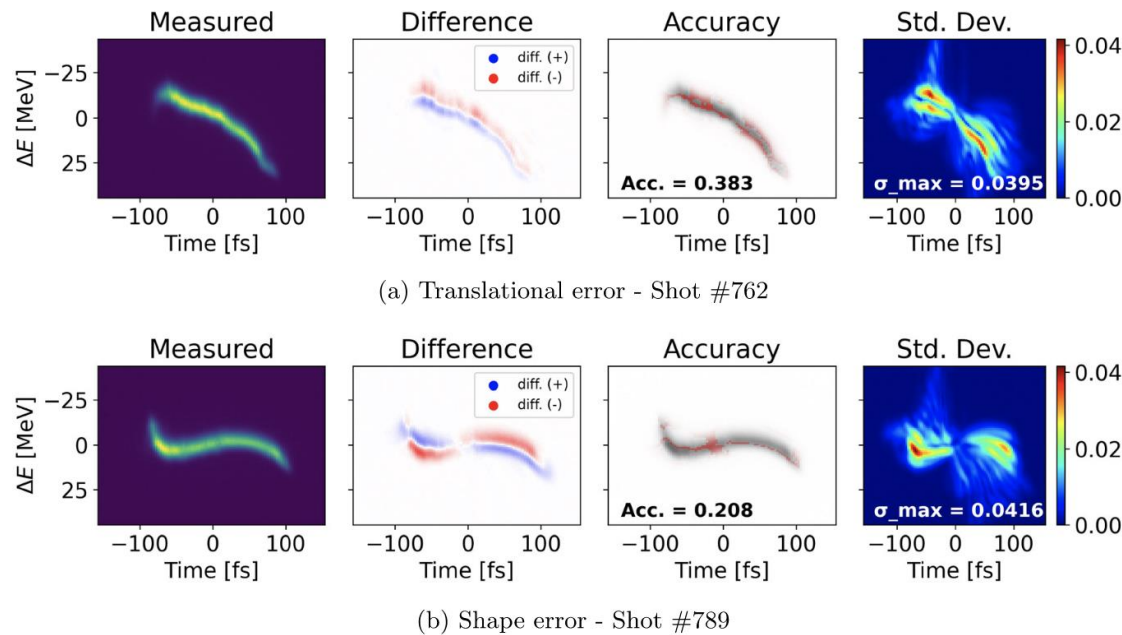
LCLS-II measured longitudinal phase space predictions.
