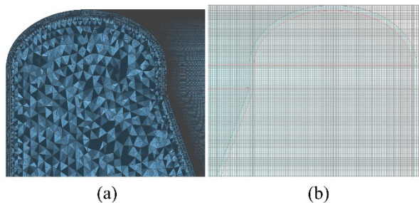
Figure 4: (a) Tetrahedral mesh used for the EM analysis and (b) hexahedral mesh used for the particle simulation.
