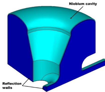
Figure 3: 1/8 symmetric HWR cavity model and reflection walls for MP simulation.
