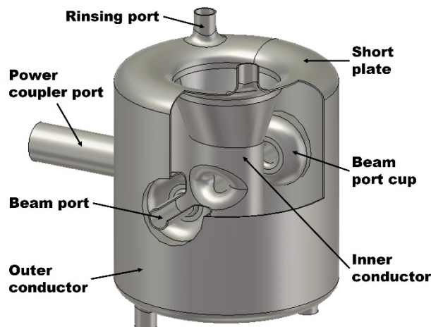
Figure 2: Cutaway drawing of the HWR designed by KOMAC.
