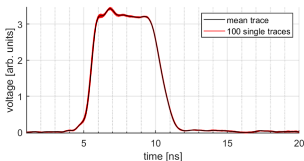
Figure 3: Single and averaged current traces measured with a 4 ns test pulse from FID GmbH.
