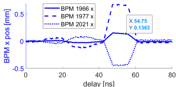
Figure 4: Measured transverse bunch positions for bunches deflected using a 2 m long stripline kicker at the European XFEL and the HV pulses shown in Fig. 3. The positions are measured at three different positions downstream the kicker position at 1960 m in the XFEL beamline, with the exact measurement positions given in the legend. For the two positions further downstream, several quadrupole magnets were used in between the kicker and the measurement position.
