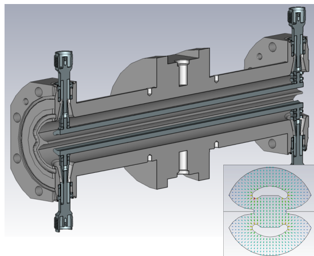
Figure 2: Mechanical design of the prototype PETRA IV stripline kicker. Inset in the lower right shows the cross section geometry.
