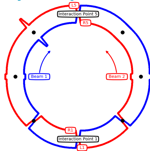
Layout of the wire installation
