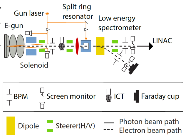
Figure 1: Schematic drawing of the low energy section, including all planned beam diagnostics. A complete overview is given in [4].
