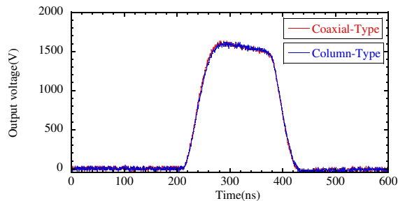
Figure 7: Measurement result of measuring two types of output voltage waveforms.
