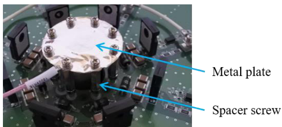
Figure 9: Picture of the gap switch test.
