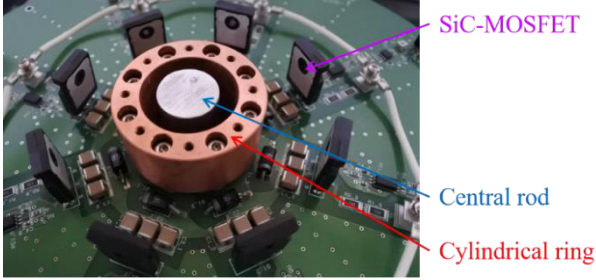
Figure 3: Picture of the coaxial-type path.
