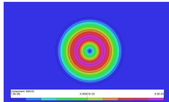
Figure 5: Contour plot of magnetic flux density of coaxial-type analysed by OPERA-2D.
