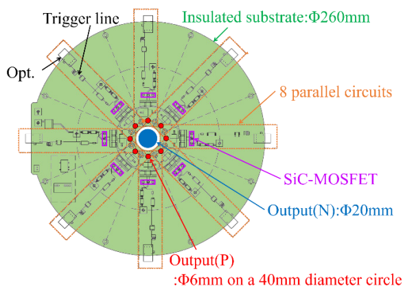
Figure 1: Conceptual diagram of the radially-symmetrical switch board.
