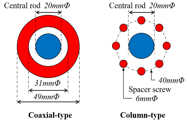
Figure 4: Conceptual view of the coaxial-type and the column-type.
