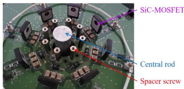
Figure 2: Picture of the column-type path.
