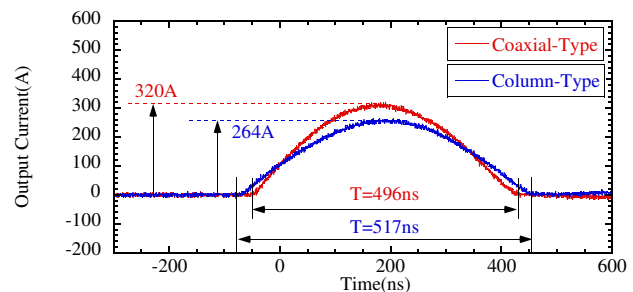
Figure 10: Current waveform measured by gap switch test.
