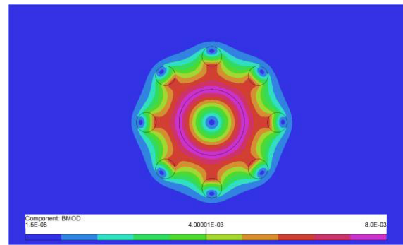
Figure 6: Contour plot of magnetic flux density of column-type analysed by OPERA-2D.
