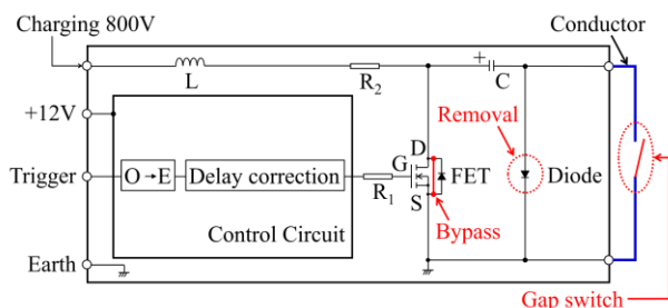
Figure 8: Block diagram of the gap switch circuit.
