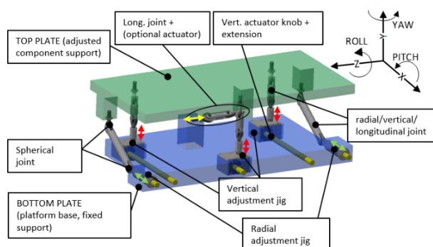
Figure 1: UAP conceptual schematic.
