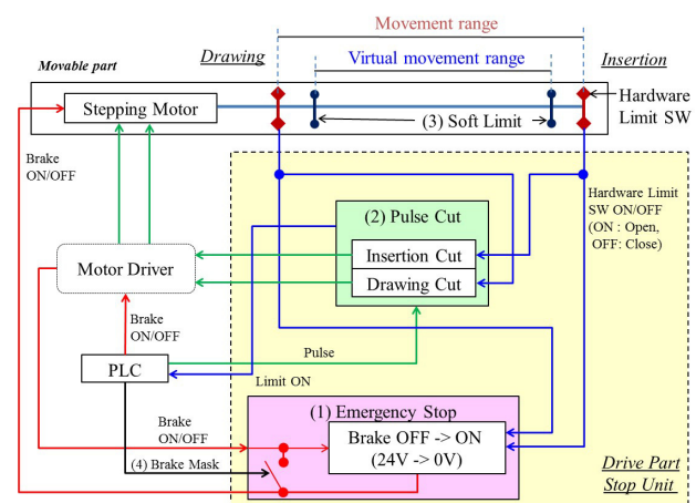
Figure 2: Configuration of improved system.
