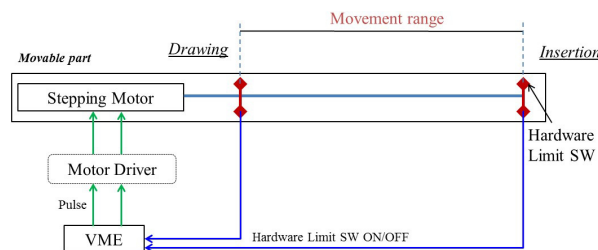
Figure 1: Configuration of existing system.
