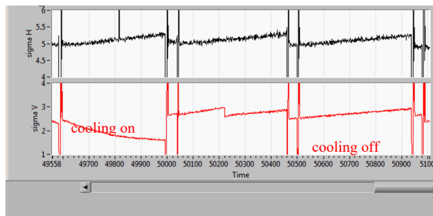
Figure 6: Beam profile measurements of vertically cooled beam.
