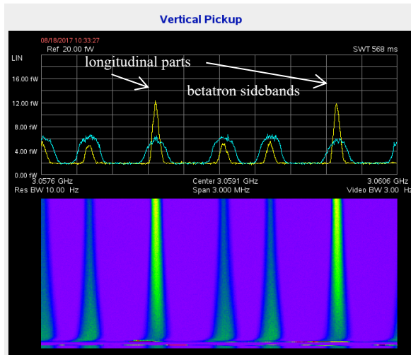
Figure 7: Difference signal of vertical plane.
