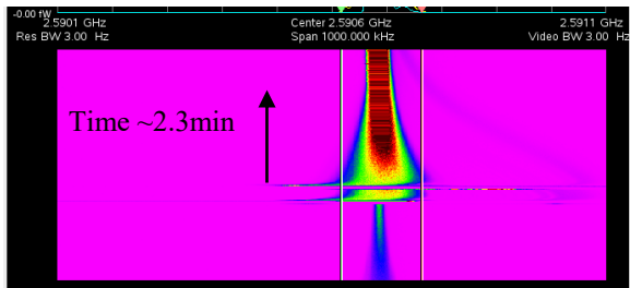
Figure 3: Longitudinal cooling of 7 \times 10^9 particles shown at the 1700 th harmonics (reduction of frequency distribution).
