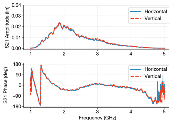
Figure 2: Open-loop measurements.
