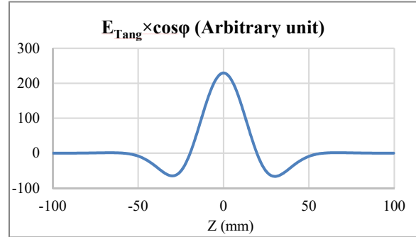
Figure 3: Tangential E-field seen by a \beta=0.78 beam with x'=50 mrad, y_0=0.01 m, equivalent to M=2127 neV-s.
