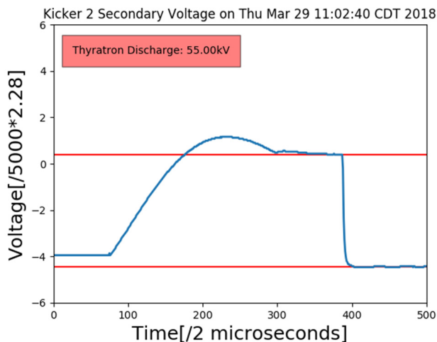
Figure 1: Blumlein charging voltage as read from the Kicker 2 transformer. Each clock tick corresponds to 2 \mu s. The numbers displayed in the vertical axis label designate the overall calibration constant applied to compensate for added cable capacitance in the DAQ system.
