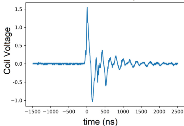
Figure 3: A voltage vs. time waveform recorded using Kicker 3's dB/dt coil.
