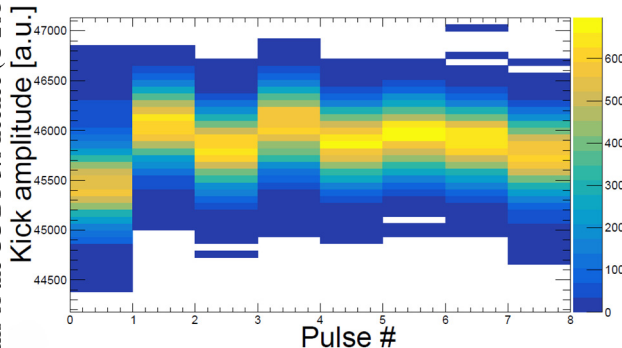
Figure 2: Amplitude of the kick strength in arbitrary units for eight pulses in a 100 Hz train.
