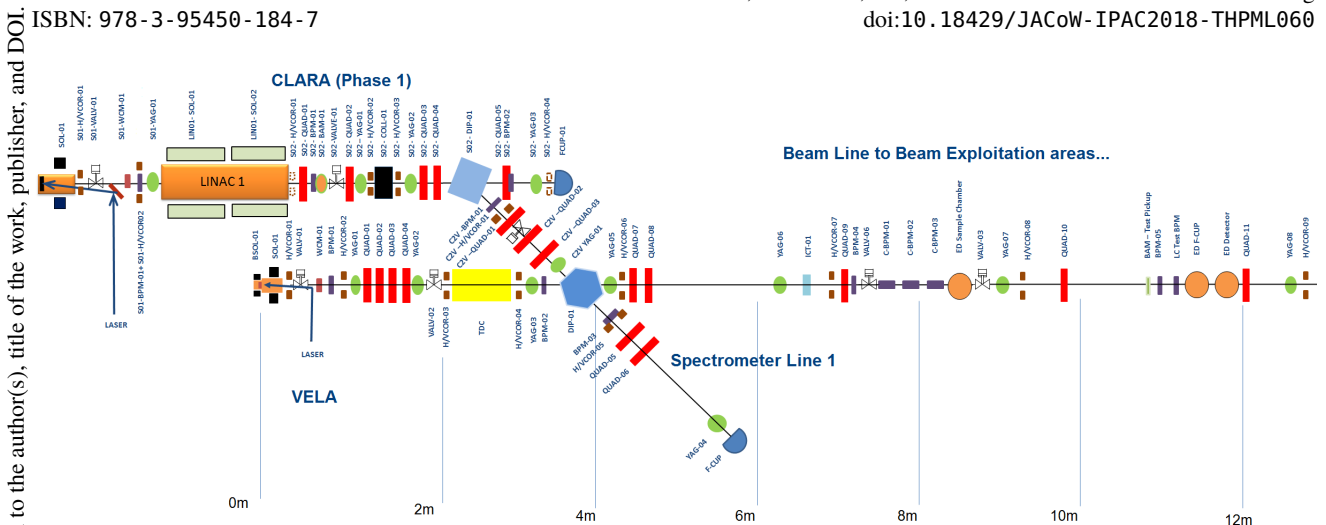
Figure 1: Schematic indicating sections of VELA-CLARA currently in the Virtual Accelerator. Not all elements have been added, but will in the upcoming future.
