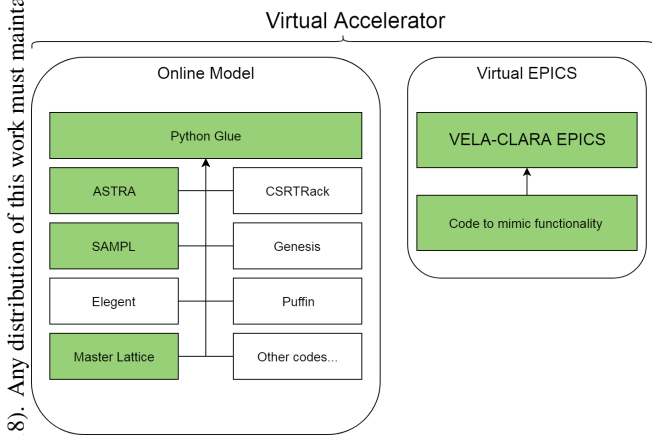
Figure 2: Block schematic indicating the components of the VA. The highlighted blocks show components already implemented.
