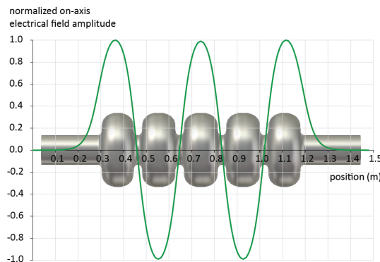
Figure 3: TM_{010} \pi -mode field profile as designed.
