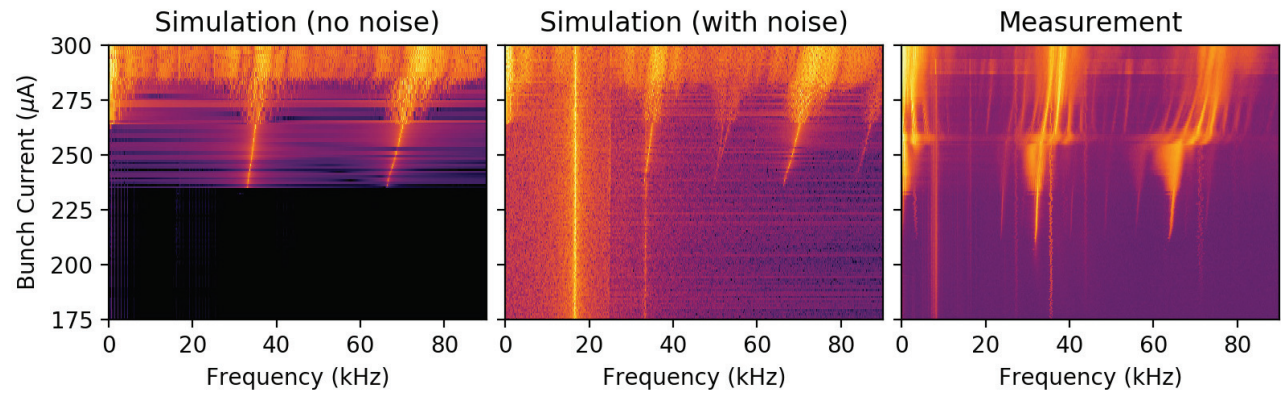
Figure 3: Spectrograms of emitted bursting coherent synchrotron radiation (see e.g. [11]). Left: Simulation data without RF noise. Center: Simulation considering RF phase noise with \sigma_q = 0.01^\circ and RF amplitude noise of \sigma_V/V = 1\% . Right: Measurement data obtained using a broad-band Schottky diode from ACST [12]. Both simulations reproduce the main frequency at f \approx 30 kHz and its harmonics. The instability threshold is 211 \mu\text{A} for the measurement and 237 \mu\text{A} for both simulations. Adding noise improves the agreement between simulation and measurement in another aspect: The unphysical drop of the background at the lowest current disappears and the minimum intensity between the peak frequencies is lowered, where an additional structure becomes visible. (See text for interpretation of current-independent f_{s,0} harmonics.)
