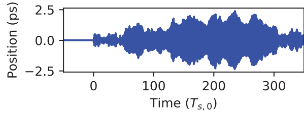
Figure 2: Evolution of the synchrotron oscillation amplitude over time. First, the simulated RF is stable. At T = 0 , white Gaussian phase noise with \sigma_q = 0.1^\circ = 0.56 ps is turned on. The natural rms bunch length is \sigma_{z,0} = 4.61 ps.
