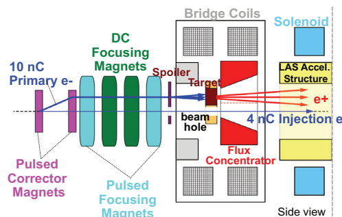
Figure 4: Positron target with a hole beside is attached in front of FC followed by LASs and solenoid coils.
