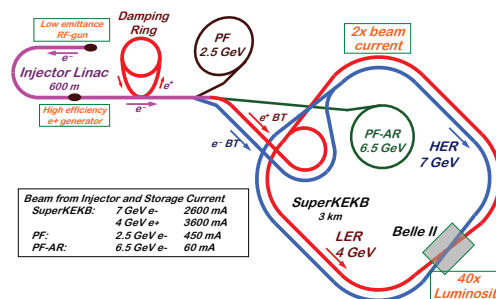
Figure 1: Layout of electron/positron injector complex with beam properties from the injector to four storage rings.
