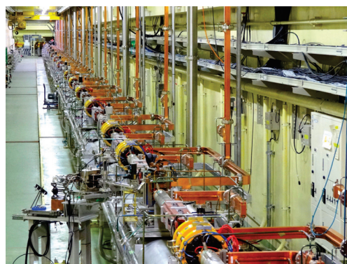
Figure 2: A typical part of the injector at the A and B sectors.
