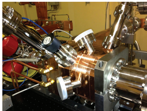
Figure 3: QWSC cavity with a high acceleration gradient.
