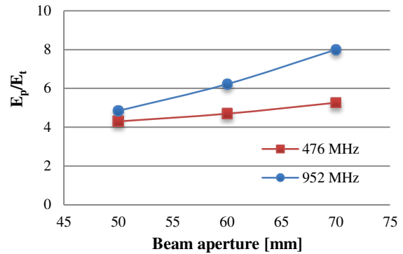
Figure 6: E_p/E_t vs. beam aperture.
