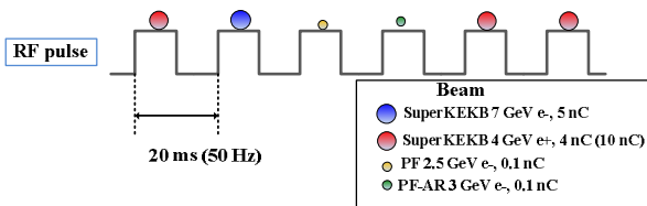
Figure 5: Schematics drawing of SuperKEKB injector linac beam operation. The beams with four different energies and amounts of charges should be managed.
