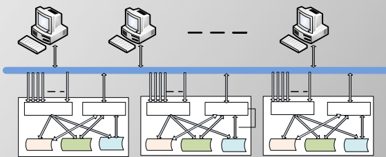
Figure 1: The structure of BEPCII real-time information system
