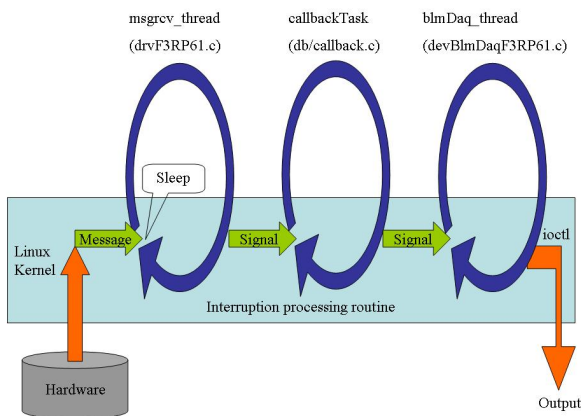
Figure 6: Thread in interruption processing routine.
