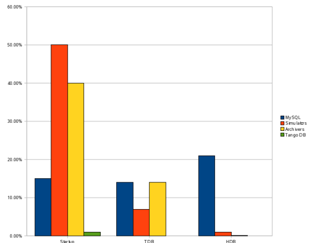
Figure 3: CPU usage vs. archiving mode
