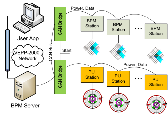
Figure 5: Hardware of the beam measurement system schematic.
