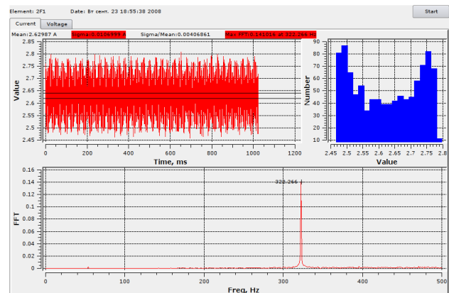
Figure 3: Analysis of the test signal from external generator. Measured values: I = 2.63 \text{ A} , n = 322 \text{ Hz} .
