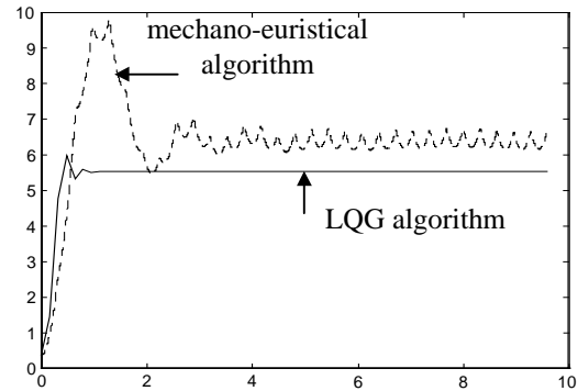
Fig. 2 Time history of controlled \theta position (minutes) without measurement noise in the presence of step velocity
