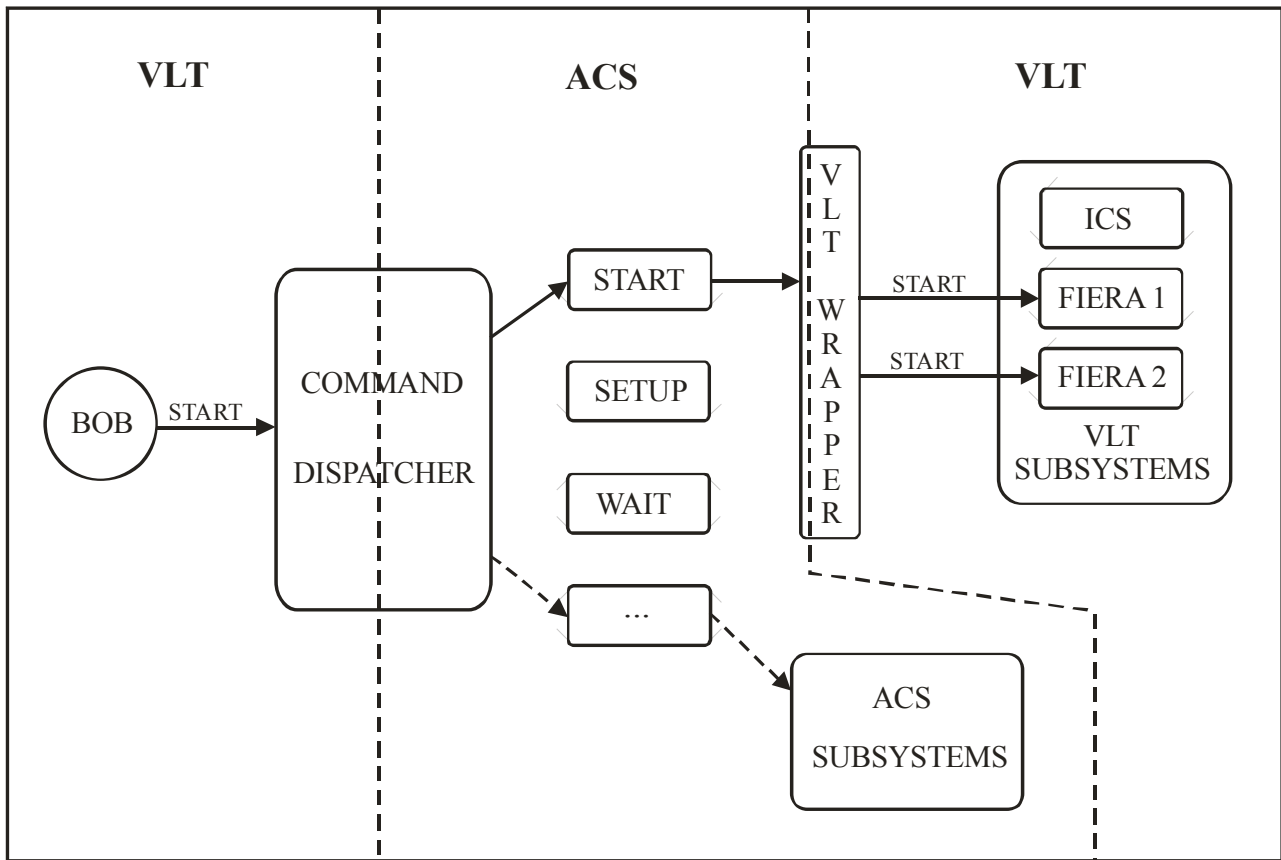
Figure 1: Overall prototype representation. The commands (e.g. START) are sent by BOB to the ACS-based OS. The VLT Wrapper allows forwarding the commands to VLT based subsystems.
