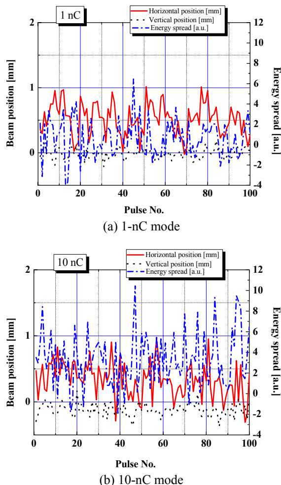
Fig. 4: Result of pulse-by-pulse measurement. (a) and (b) show the result of 1-nC (single bunch) and 10-nC (two-bunch) operation modes respectively. Solid (red), dotted (black) and broken (blue) lines mean horizontal, vertical beam positions and energy spread, respectively.
