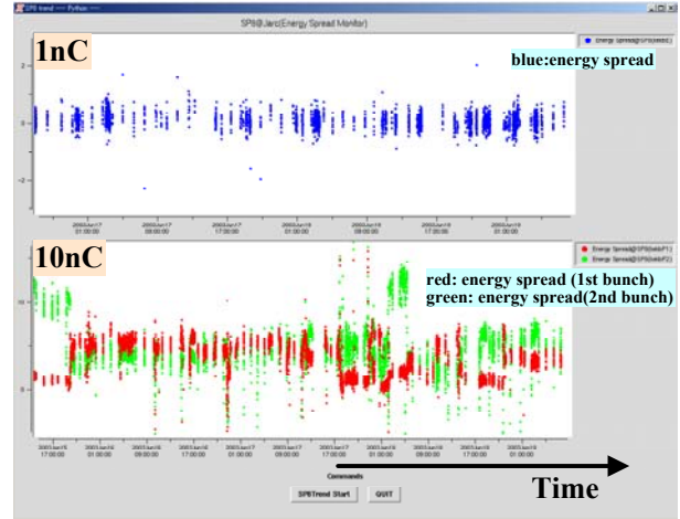
Fig. 3: Software GUI
