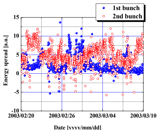
Fig. 5: Result of long-term measurement. Filled circle (blue) and open circle (red) show the energy spread of 1st and 2nd bunch respectively.
