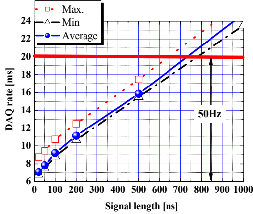
Fig. 2: Result of data acquisition speed. Square (red), triangle (black) and circle (blue) mean maximum, minimum and average data acquisition time.
