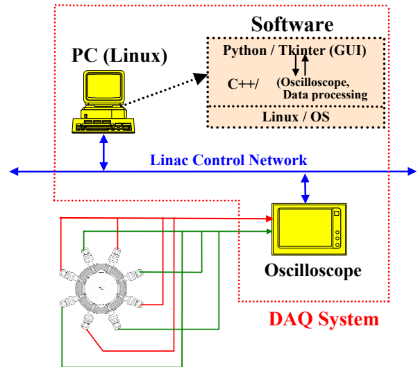
Energy Spread Monitor (ESM)
