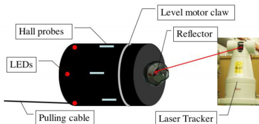
Figure 2: Mole equipment
