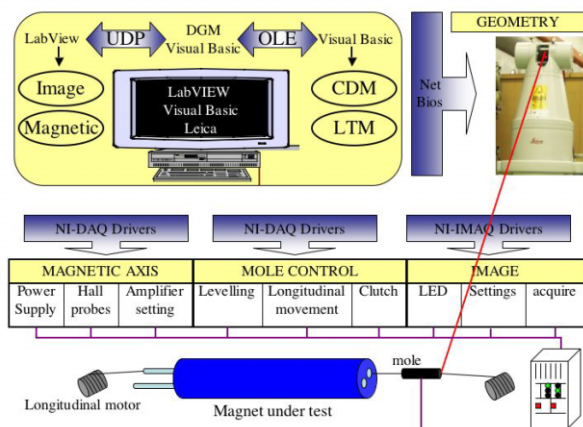
Figure 3: Measuring system architecture
