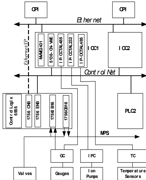
Figure 4: Architecture of vacuum control system of storage ring
