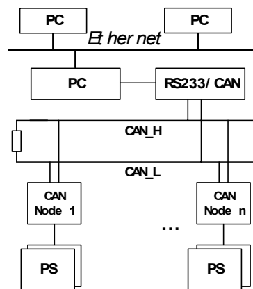
Figure 1: System architecture before upgrade
