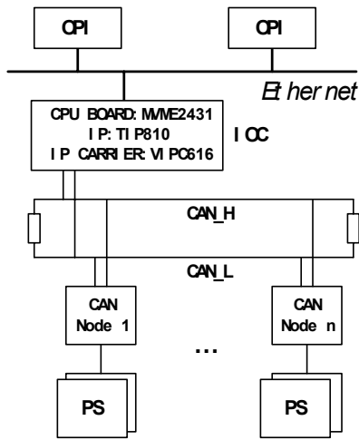
Figure 2: System architecture under EPICS
