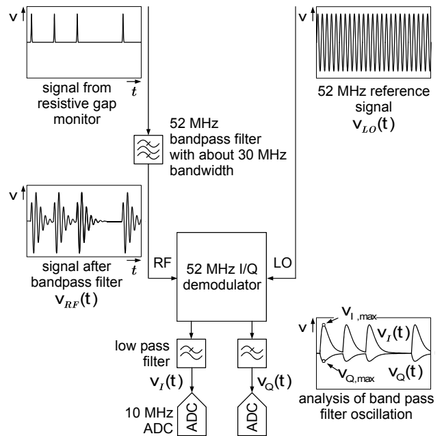
Figure 1: Measurement principle
