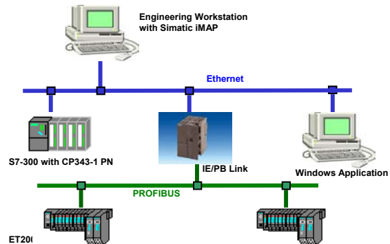
Figure 3: PROFINet Test System.
