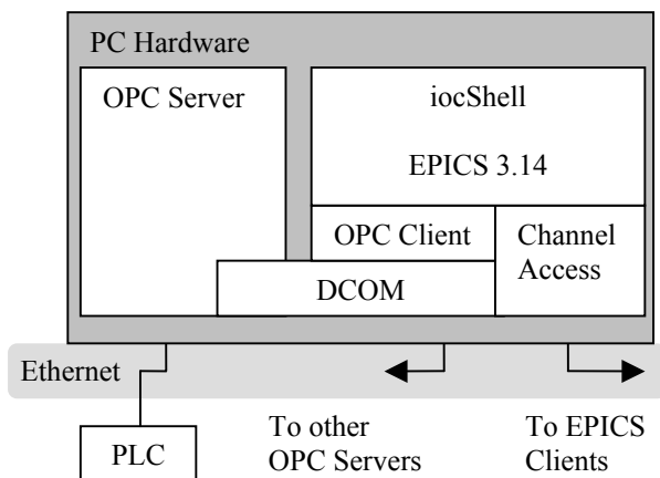
Figure 3: Data Flow from the PLC through the OPC Server to EPICS
