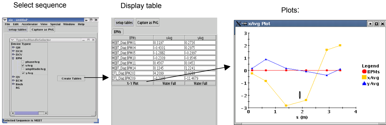
Fig. 5: The XIO application, progression from accelerator sequence selection to device type selection to signal type selection to data monitoring (tabular + plots).
