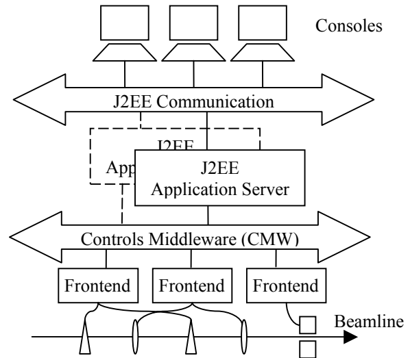
Figure 1: The CESAR 3-tier architecture
