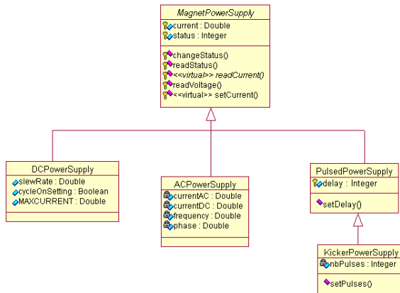
Figure 5: Magnet power supply class diagram.
