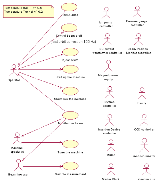
Figure 1: Main use case diagram.
