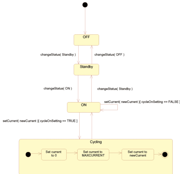
Figure 6: DC magnet power supply state machine.
