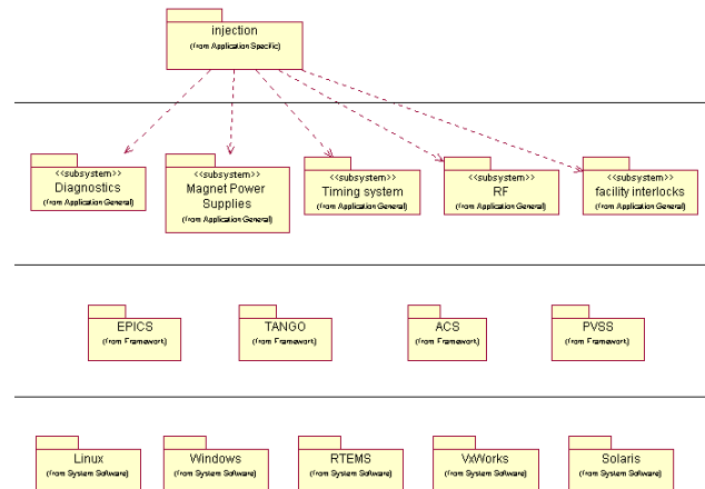
Figure 4: Layered architecture.
