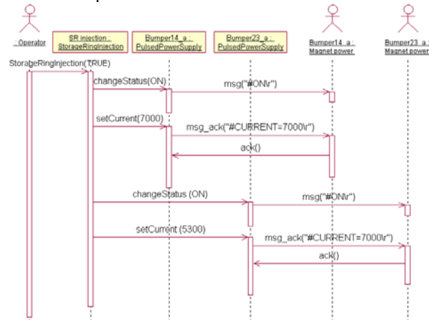
Figure 7: Sequence diagram for the injection in the storage ring.
