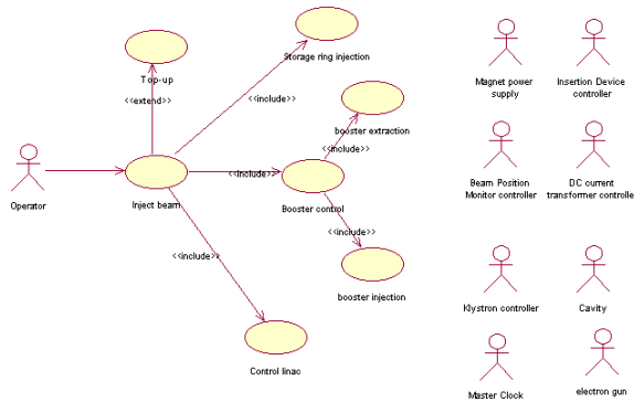
Figure 2: Inject Beam use case diagram.
