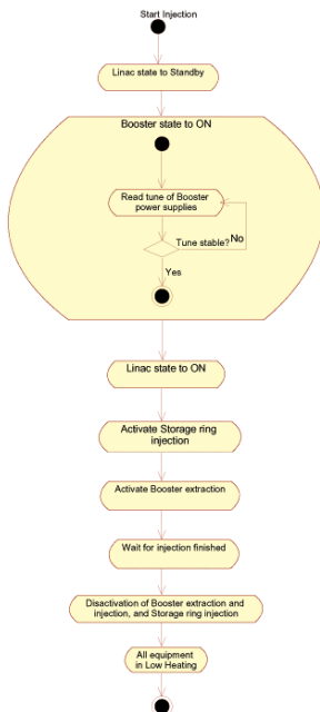
Figure 3: Activity diagram for the Inject Beam use case.
