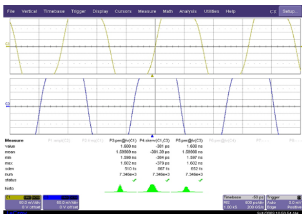
Figure 2: Jitter test of Infineon V23818-N305-B57 transceiver
