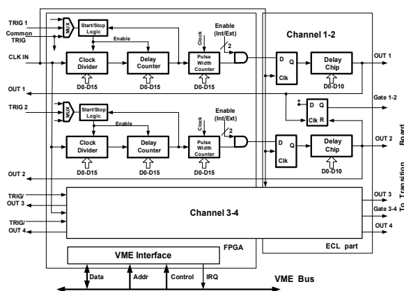
Figure 4: Functional scheme of the 4 Channel Timer
