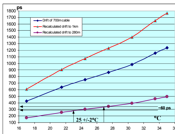
Figure 3: Propagation delay drift of OM3 fibre as a function of temperature
