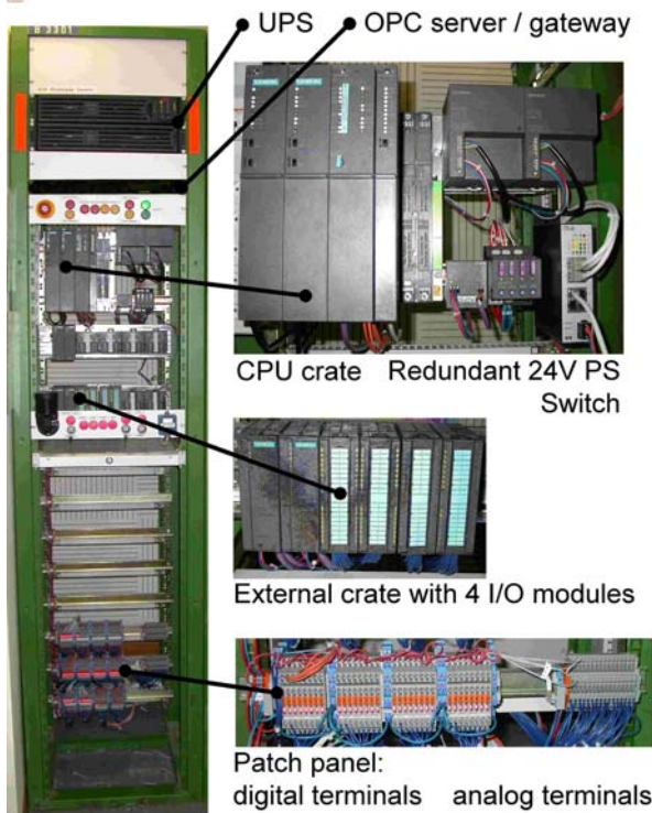
Figure 3: Hardware Layout of a Detector Safety Unit.
