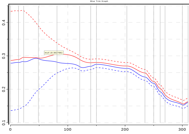
Figure 4: Blue Tunes: No B_2 feed-down (Dashed), with B_2 feed-down correction (Solid) assuming \Delta x = 2.15\text{mm}
