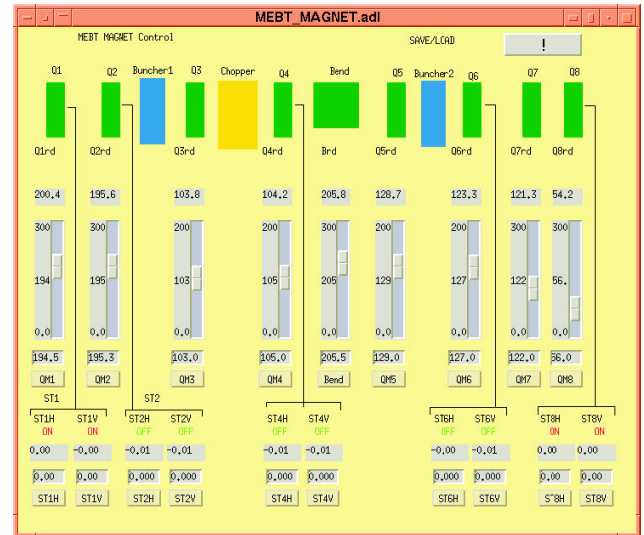
Figure 2: Control panel for the MEBT power-supplies
