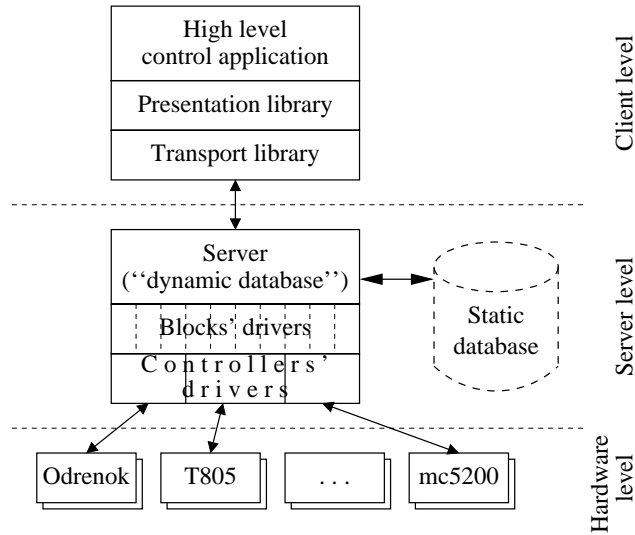
Figure 3: Structure of the current clients ↔ server ↔ hardware system.
