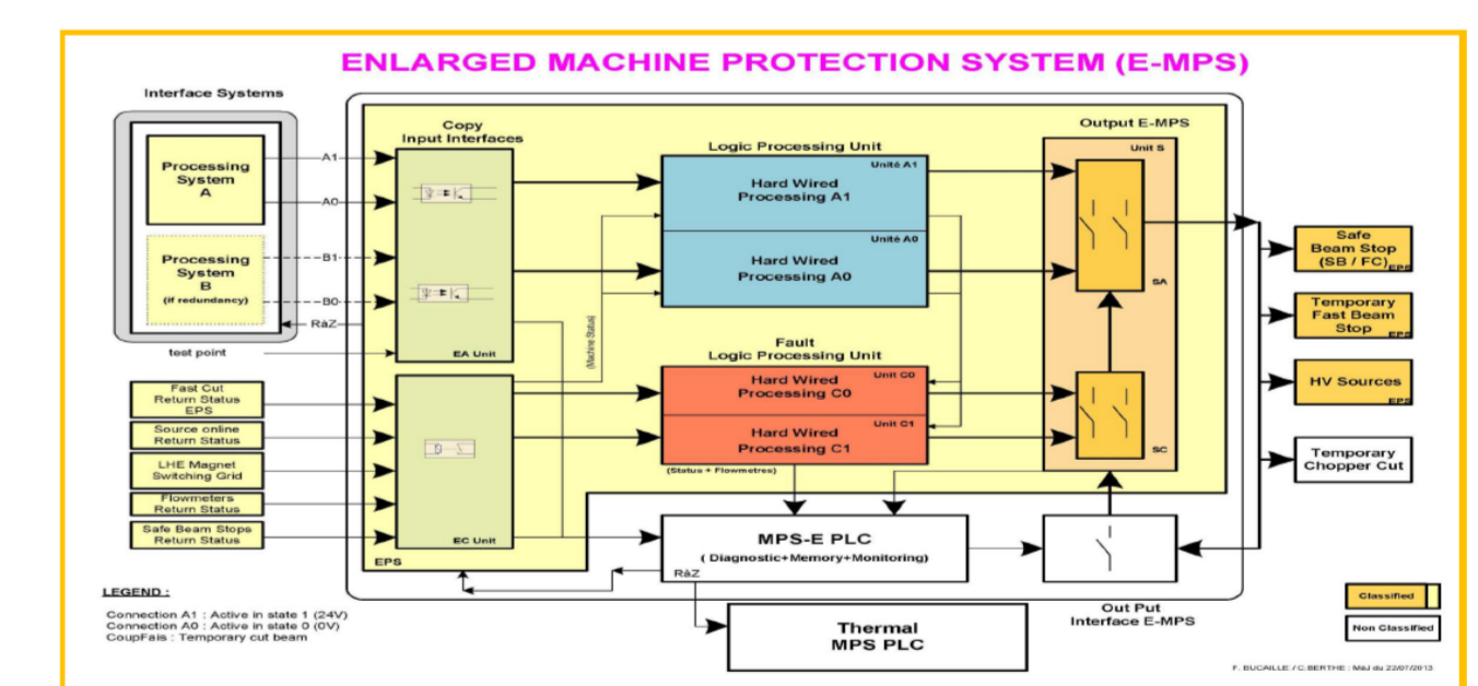
Redundant hard-wired system
