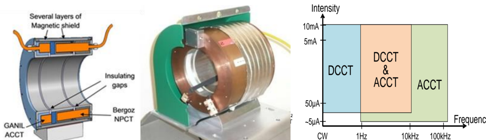
ACCT/DCCT bloc section and operating range
