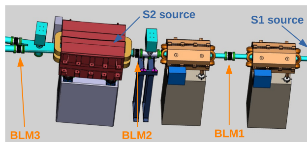
Figure 5: A section of the HADES beam line consisting of a quadrupole doublet and a switching magnet. The beam comes from the right.
