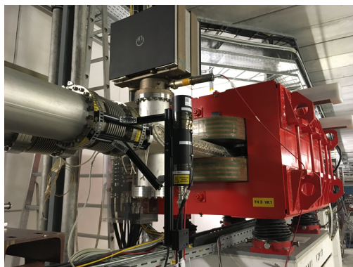
Figure 2: BLM (the black cylinder) behind a switching magnet (in red). The beam aperture is limited due to the dipole vacuum chamber in vertical direction.
