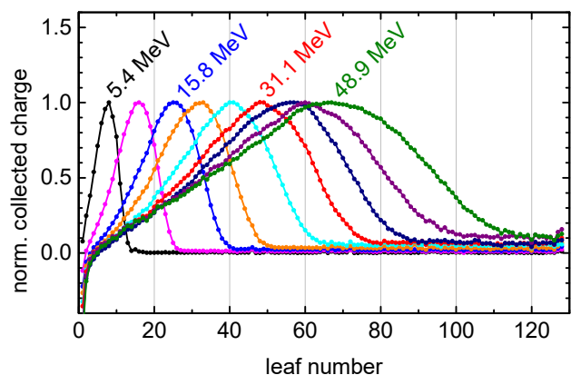
Figure 4: Electron distributions for different beam energies as recorded by the MLFC.
