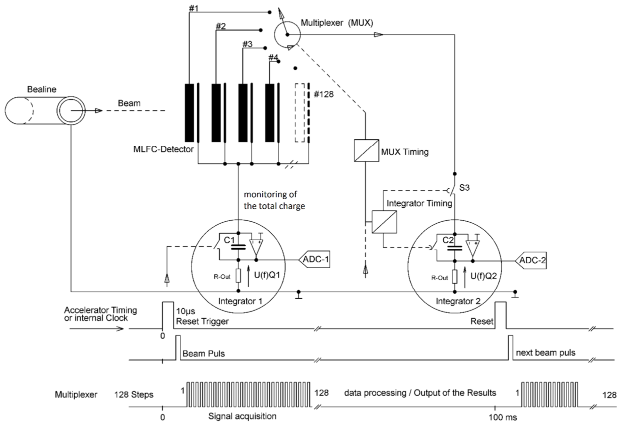
Figure 2: Schematic diagram for read out of the MLFC.
