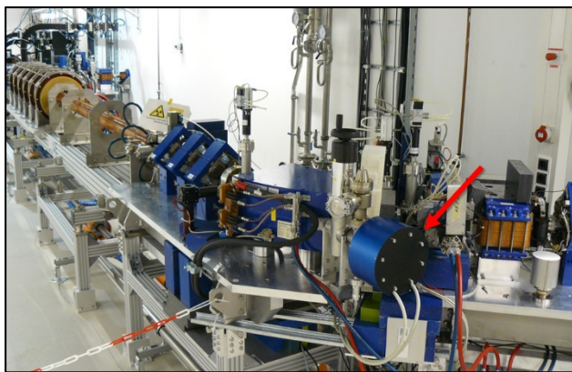
Figure 6: MLFC in its housing mounted at the end of the accelerator structure (red arrow) as replacement of a beam dump.
