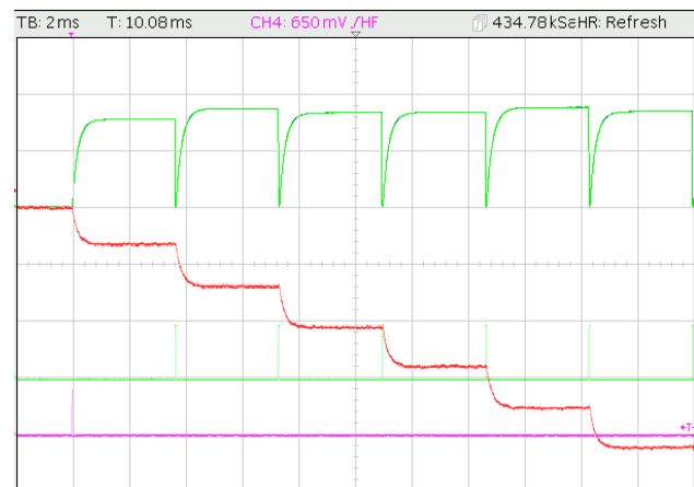
Figure 3: Oscillogram of signal from Integrator 1 (red) and Integrator 2 (upper green) during readout of the MLFC.
