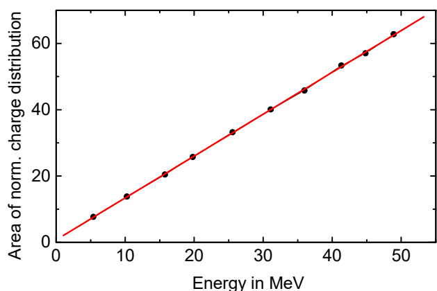
Figure 5: Calibration curve. Red line linear fit to data.
