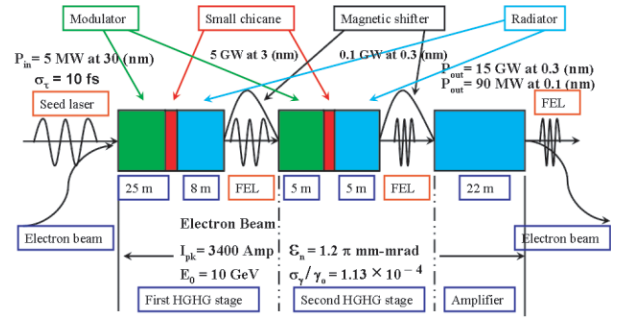
Figure 1: Schematics of an HHG seeded cascaded HGHG FEL. In this scheme an HHG seed of 30 nm is used. After two stages of HGHG and a final amplifier, we obtain 15 GW at 0.3 nm, and 90 MW at 0.1 nm.
