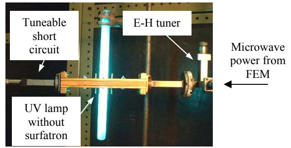
Figure 7: 100μs pulses fill a 30cm UV tube.
