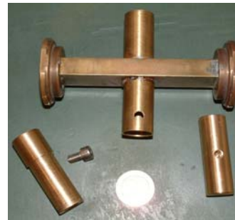
Figure 9: X-Band chemical synthesis reactor.
