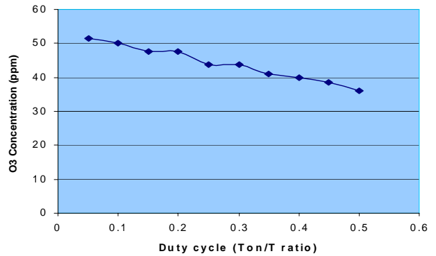
Figure 8: Experimental measurements to investigate the effect of duty –cycle on Ozone production.
