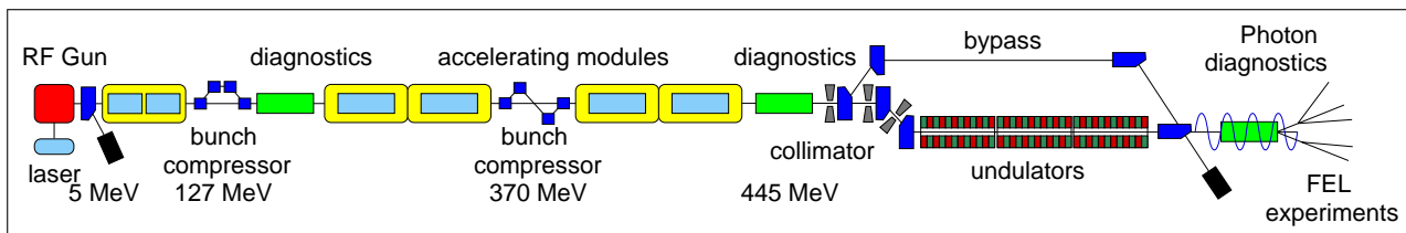
Figure 1: Schematic overview of the VUV-FEL linac (not to scale). Beam direction is from left to right, the total length is about 250 m.
