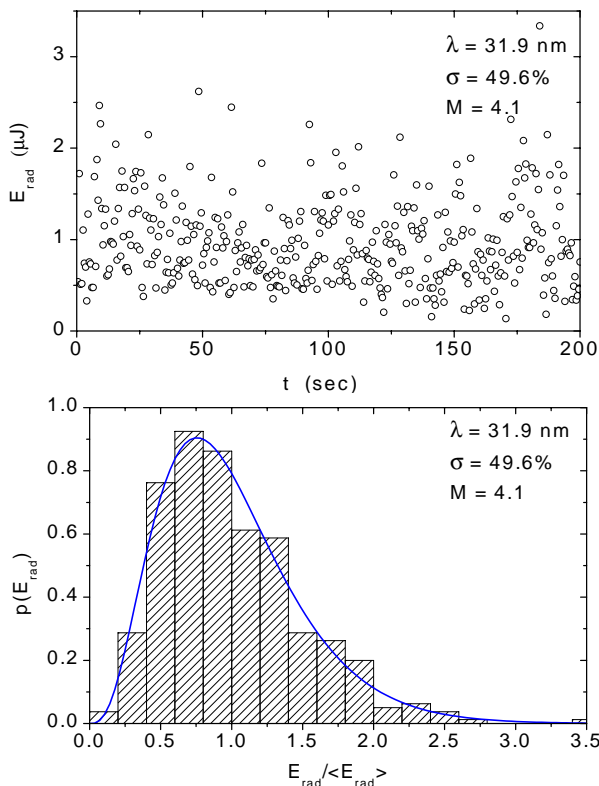
Figure 4: Example of the measured energy in the FEL radiation pulses for a certain period of time (top). The same data normalized to the average energy are shown as a histogram giving the probability distribution (bottom).[10] The rms energy fluctuation \sigma of 49.6% gives the number of lasing modes M of 4.1, which determines the Gamma-distribution drawn as a solid line. (The data bins are scaled such that the area is equal to the integrated Gamma-distribution.)
