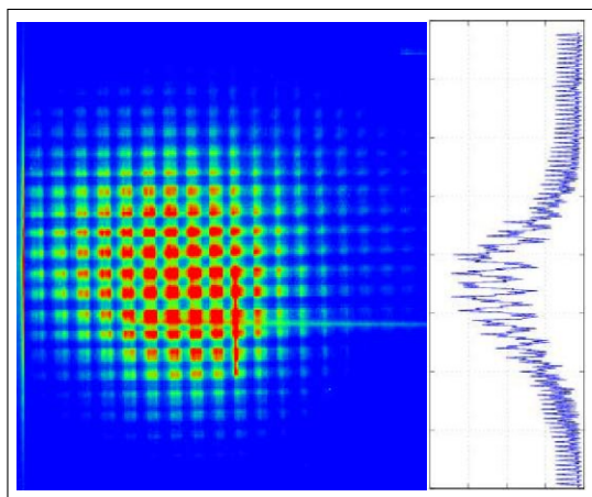
Figure 2: Image of a the FEL beam on a Ce:YAG crystal (single shot) and its projection.[10] The gold mesh of the radiation detector in front of the screen is visible and allows to estimate the width of the beam to 3 mm (fwhm) at 18.5 m distance from the undulator (wire distance 0.31 mm). This results in an angular divergence of 160 \mu\text{rad} (fwhm).
