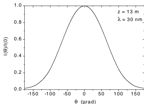
Figure 3: Simulated intensity distribution of the FEL radiation in the far zone.[11] The angular divergence is 150 \mu\text{rad} (fwhm) in good agreement with the measurement.
