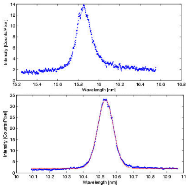
Figure 7: Measured average spectra of the second (top) and third (bottom) harmonic of 32 nm. The center wavelengths are 15.86 nm and 10.53 nm respectively.
