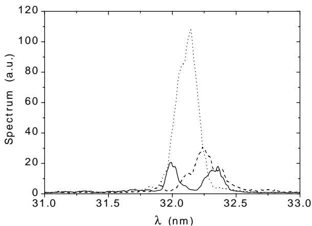
Figure 5: Example of three measured single shot spectra with different line shapes.[10] The center wavelength is 32 nm, the spectral width typically 0.25 nm.
