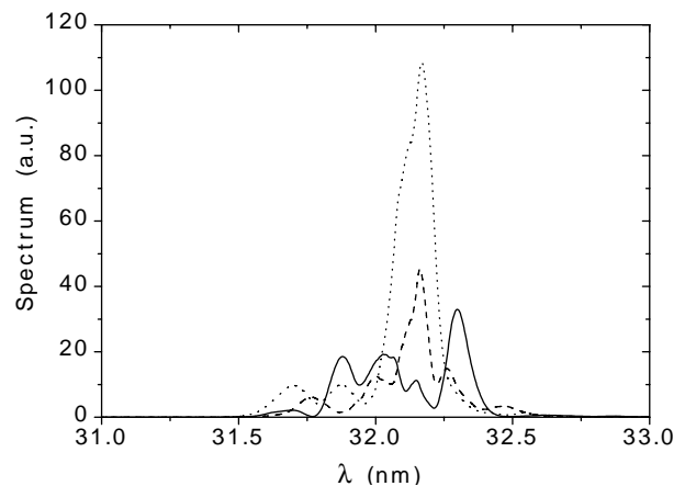
Figure 6: Simulation of the spectra operating in the exponential regime.[11] They are in good agreement with the measurements.
