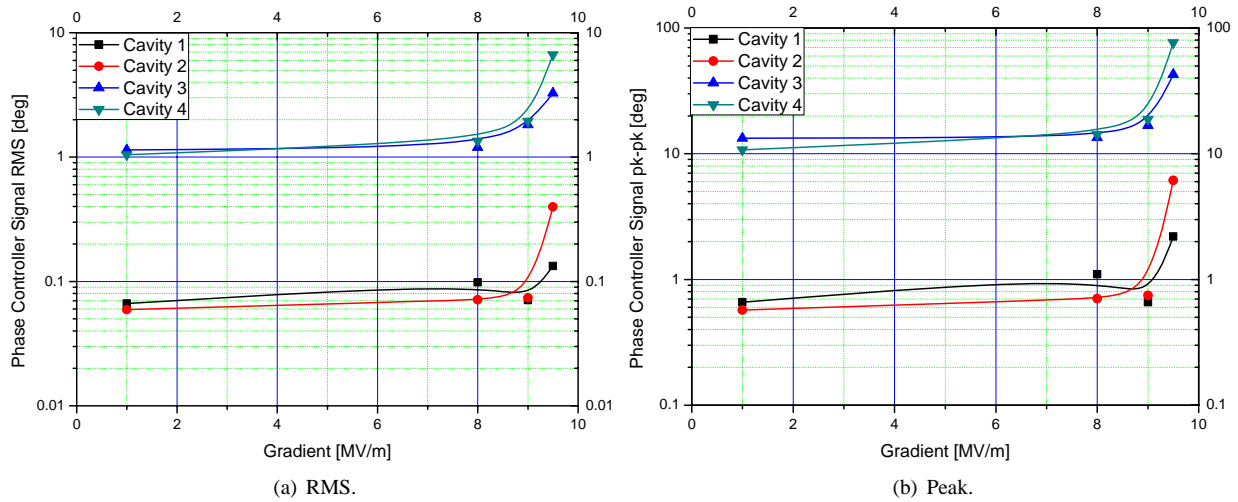
Figure 6: Variation of RMS- and Peak-values of phase controller signal with the gradient for all cavities.
