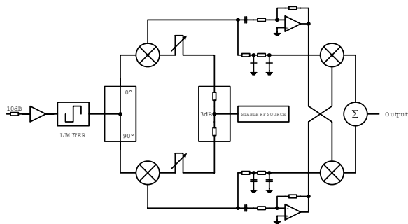
Figure 8: Circuit of the used Resonance-Monitor.
