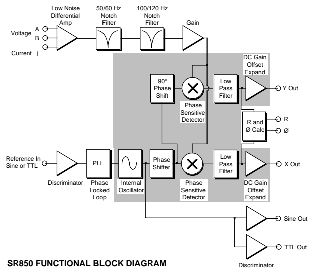
SR850 FUNCTIONAL BLOCK DIAGRAM
