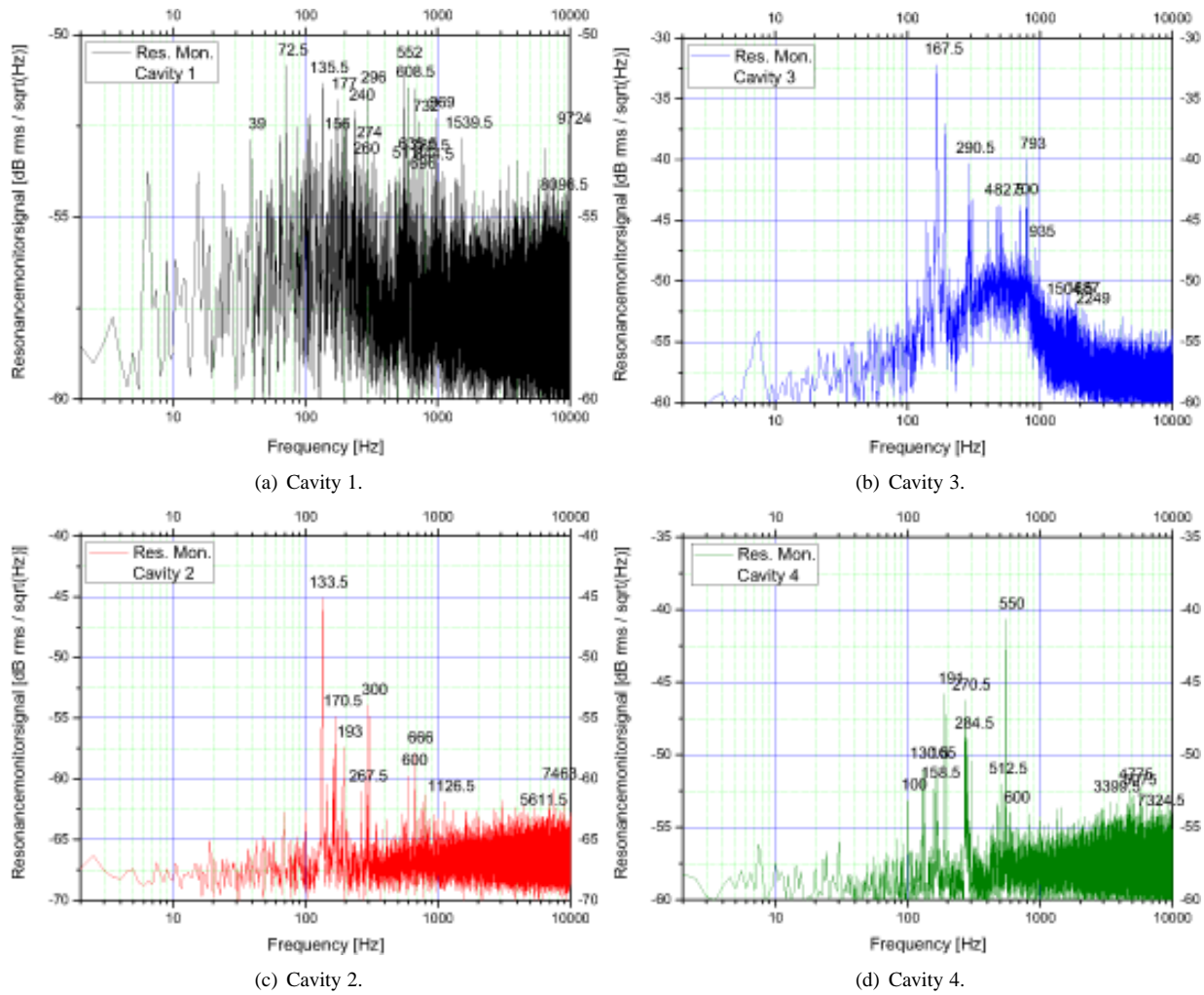
Figure 9: Power spectral density spectra of resonance monitor output signals for cavity 1 to 4.
