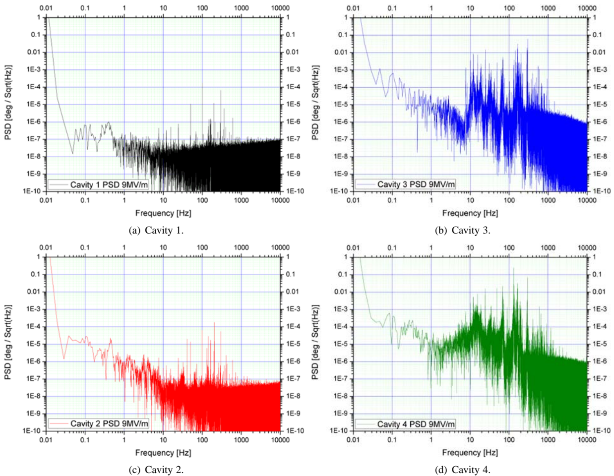
Figure 7: Variation of power spectral density of phase controller signal for cavities 1 to 4 at 9MV/m gradient.
