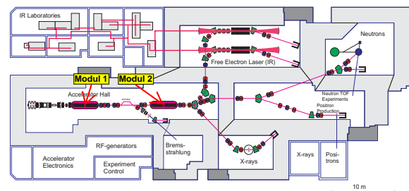
Figure 1: Radiation Source ELBE - 40 MeV, 1mA CW LINAC, Location of Cryogenic Modules.
