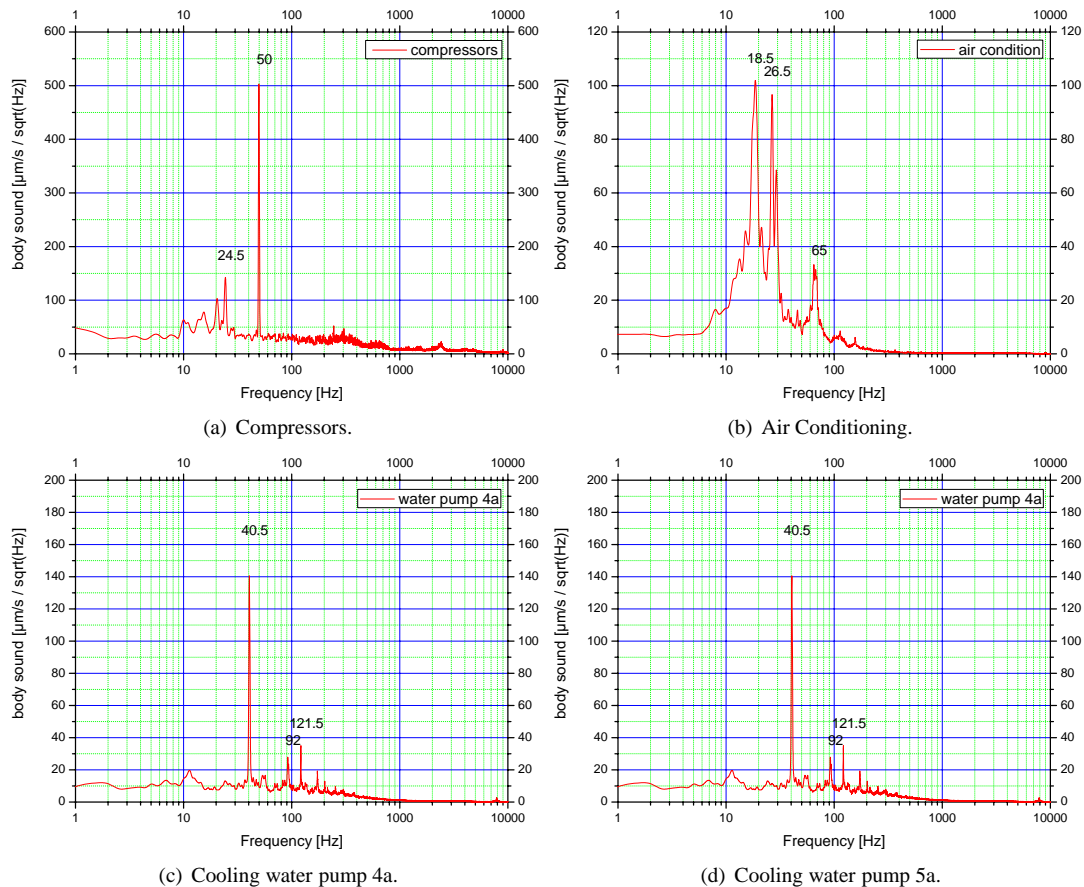
Figure 12: Some power spectral density spectra of body sound sources at ELBE.
