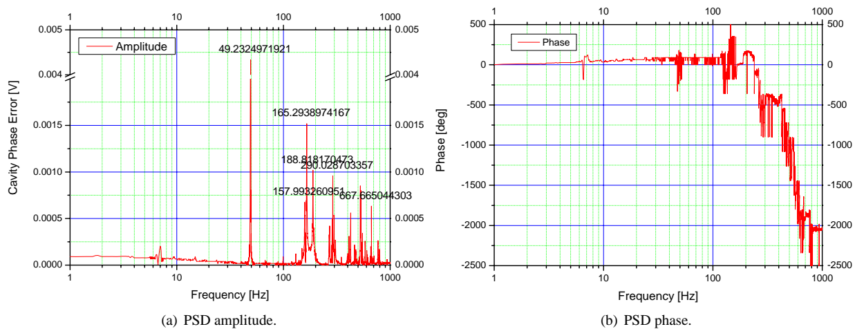
Figure 11: Amplitude and Phase variation of power spectral density due to the Lorentz force excitation of mechanical eigenmodes.
