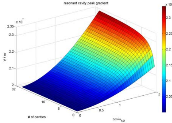
Figure 4: Gradient imbalance as function of A_{\Delta f} and N, f_m = 100 Hz
