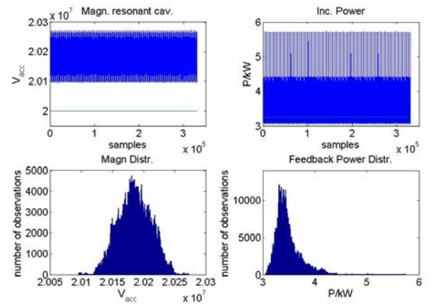
Figure 5: Example for case 2 with detuning of full bandwidth in the high frequency range.
