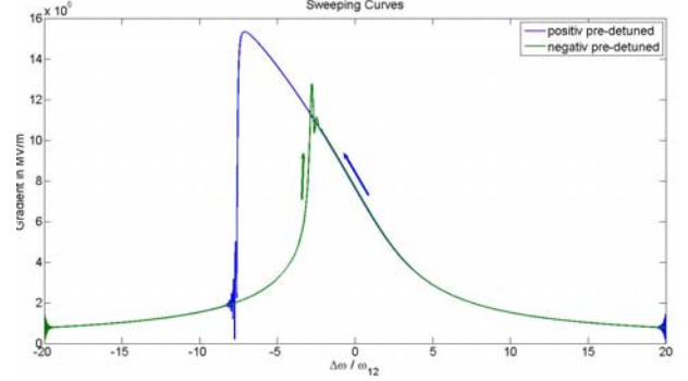
Figure 7: Sweeping curves in single cavity.
