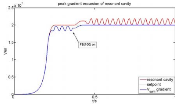
Figure 3: Gradient imbalance of resonant cavity for a feedback gain of 100 and the vector sum of 8 cavities.
