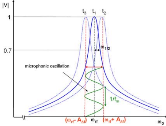
Figure 1: Resonance curve displacement due to microphonic vibrations.
