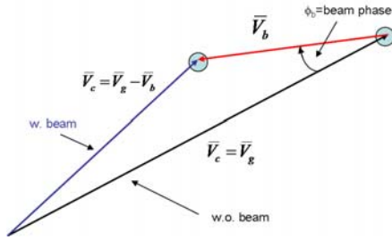
Figure 6: Calibration with beam induced field.
