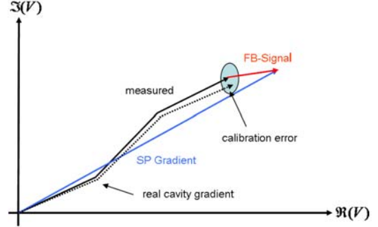
Figure 2: Influence of the calibration error on the feedback signal
