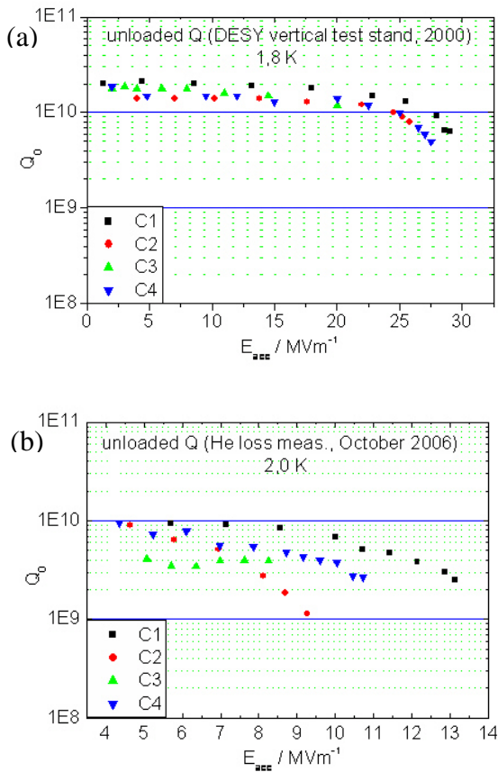
Figure 2: Acceleration gradient of the ELBE cavities after fabrication (a) and after He-Tank welding and four years operation (b)
