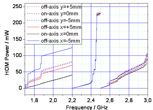
Figure 6: Total damped power of HOM at typical ELBE beam parameters ( 20 MeV, 240 \mu A)
