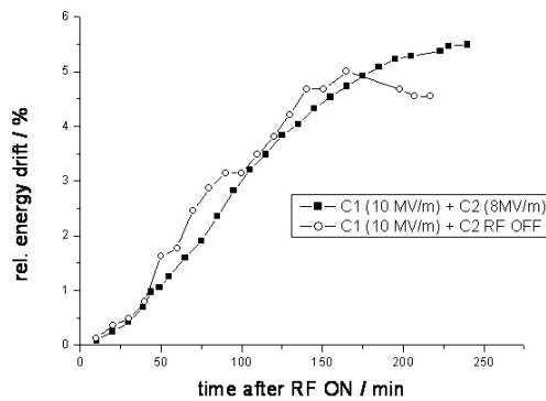
Figure 5: Drift of beam energy during the first hours after switch on of RF in ELBE linac module one. The energy drift during operation with two cavities (full quads) and with only cavity 1 (open circles) were measured.
