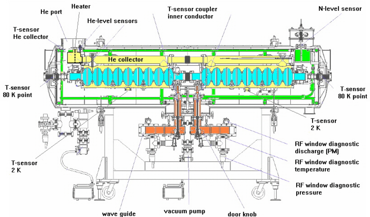
Figure 1: The ELBE linac module for cw operation
