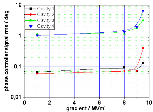
Fig 4: Rms of the phase controller signal distribution versus acceleration gradient for all ELBE cavities
