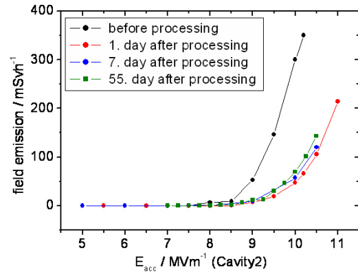
Figure 3: Stable reduction of field emission level by pulsed RF processing
