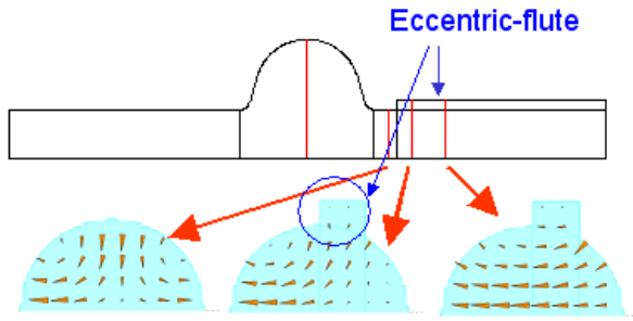
Figure 3: The principle of the EFB. The arrows show the excited electric field at each cross section.
