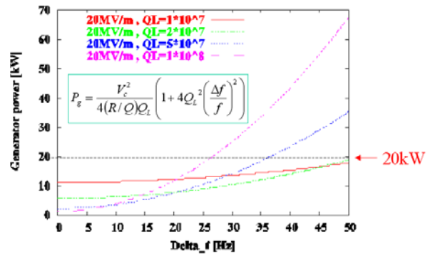
Figure 13: Input power vs. cavity detuning, \Delta f , corresponding to the several Q_L 's.
