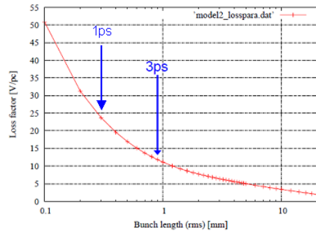
Figure 6: Loss factor of KEK-ERL model-2 cavity.
