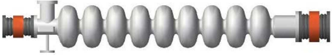
Figure 1: Conceptual view of the KEK-ERL model-1 cavity.
