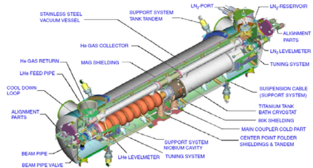
Figure 10: ELBE cryomodule.
