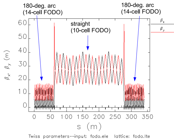
Figure 10: Betatron functions for the 1st loop.
