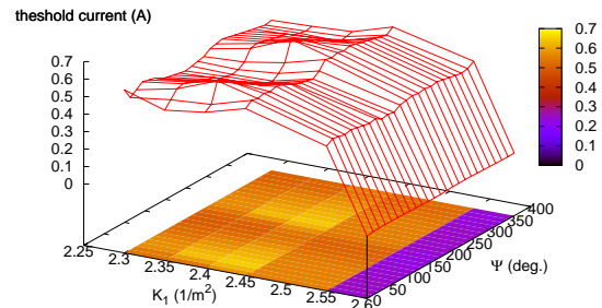
Figure 3: BBU threshold current for the 5 GeV ERL with Model-2 cavities as a function of beam optics, strength of the linac quadrupoles, K_1 , and phase advance of the return loop, \Psi .
