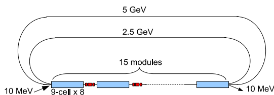
Figure 9: A 5 GeV ERL light source with a 2-turn configuration.
