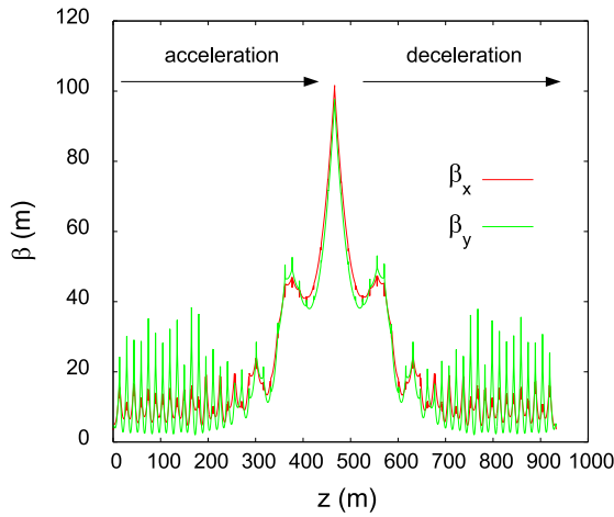
Figure 5: Optimum betatron envelopes obtained from the ‘minimum beam size’ scheme.
